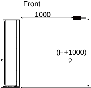
Sound pressure level measurement (unit: mm)
